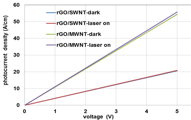
Figure 3 current density measured for rGO/SWNT and rGO/MWNT composites on spin coated films (thickness ~50 nm) irradiated by of infrared laser
