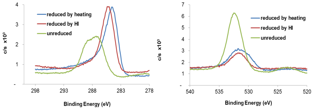
Figure 2 XPS spectrum, C1s (left side) and O1s (right side) for thermally, chemically reduced and unreduced GO films
